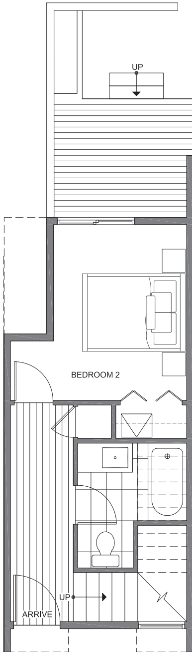
FIRST FLOOR
